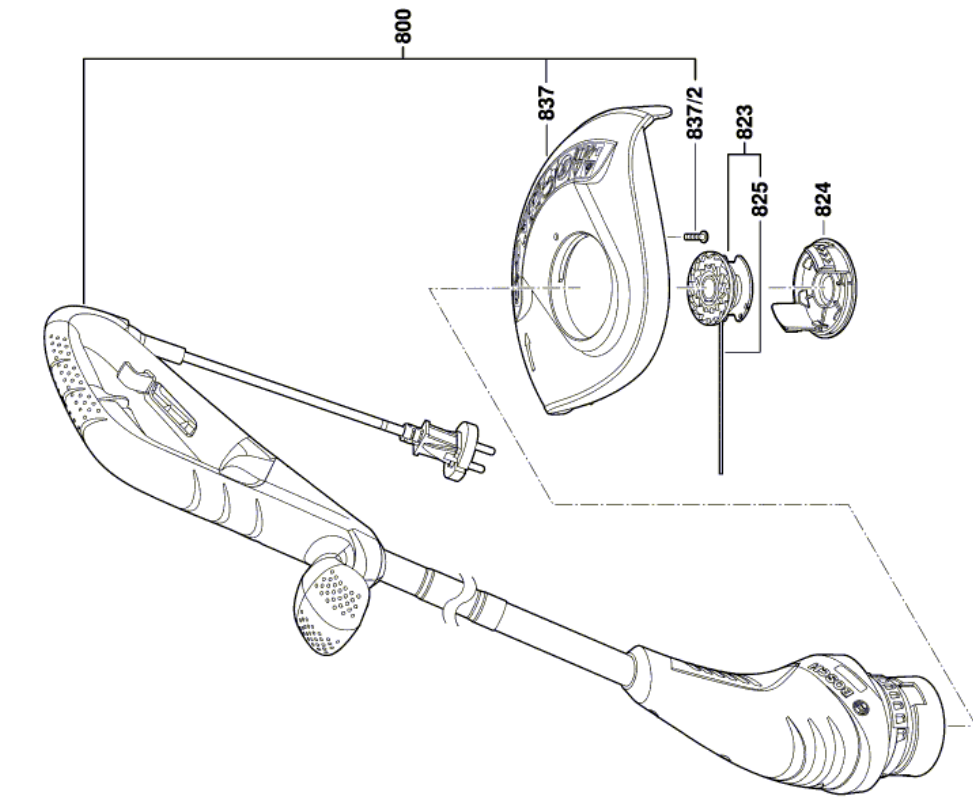
3 600 HA5 000 Stand } Issue } 13-12-12 Fig./Abb. 1
